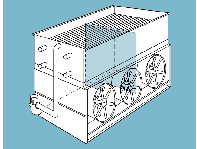
Internal Baffles
